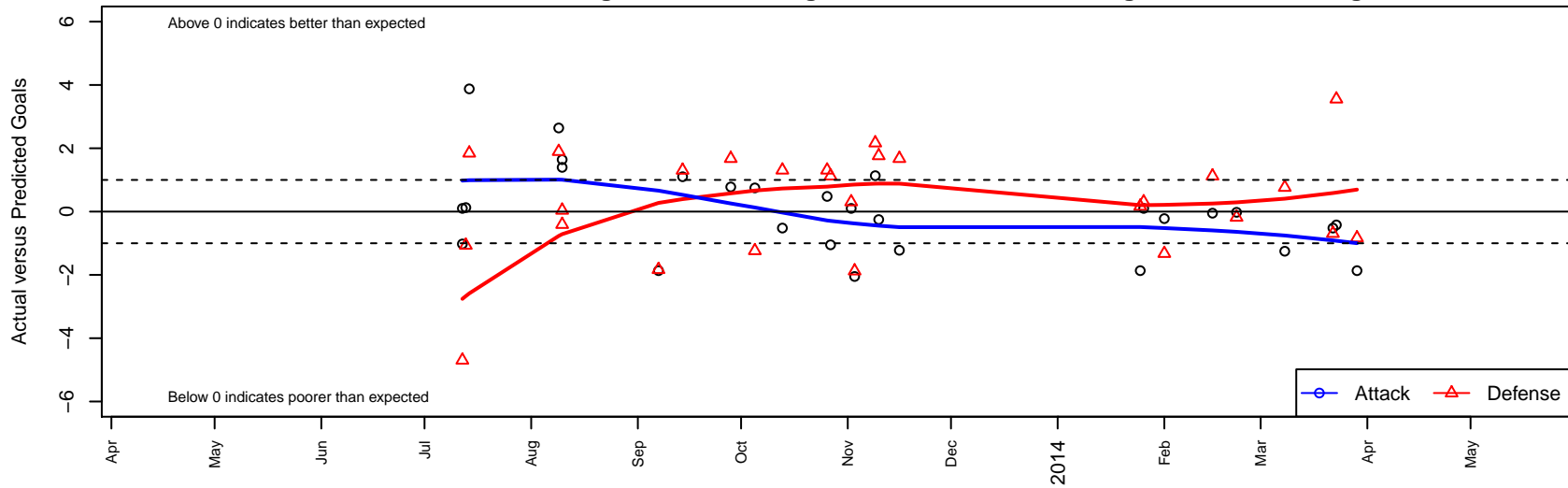
FWFC White B02 Dots are actual minus expected GF (blue circles) and GA (red triangles). Blue line is smoothed change in attack strength. Red is smoothed change in defense strength.
